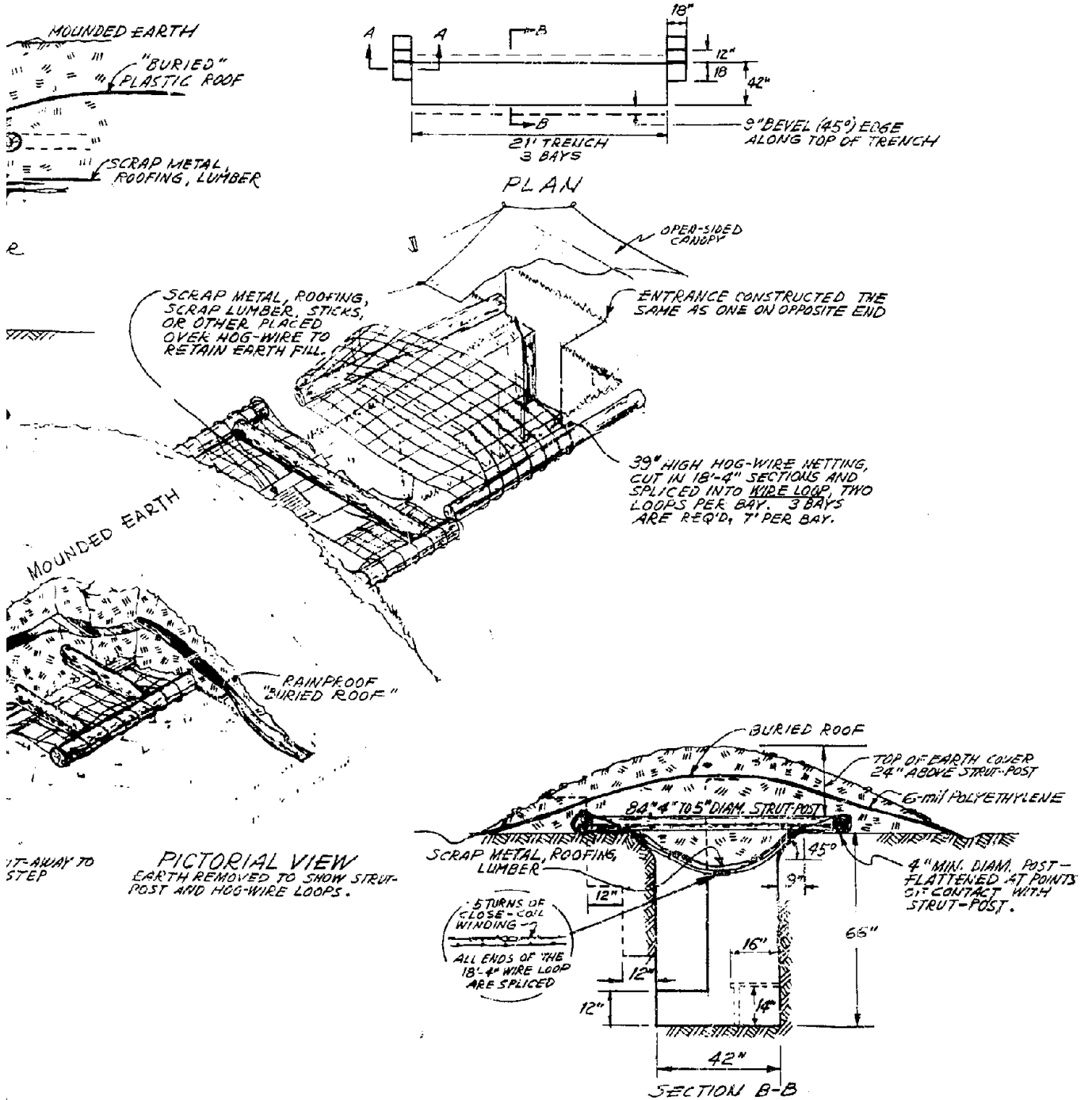
Fig. A-3.1. Catenary wire roofed shelter - basic design.
